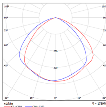
High Bay HPI 400W
