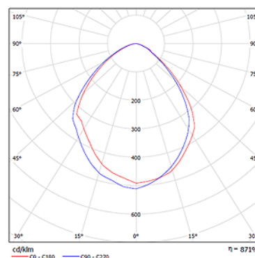
High Bay HPI 250W
